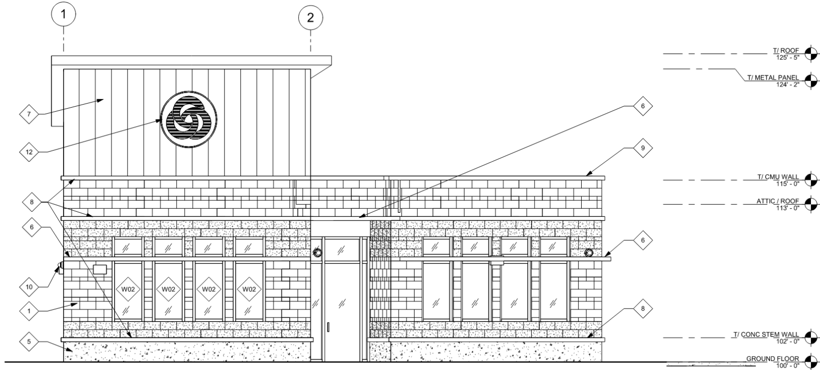
South Elevation – Operator Break Building
