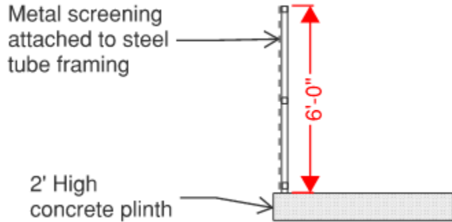
Section through screening
