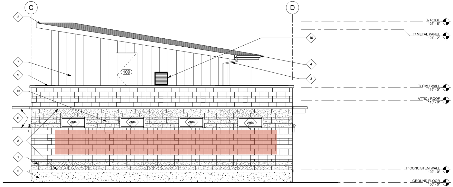
East Elevation – Operator Break Building
